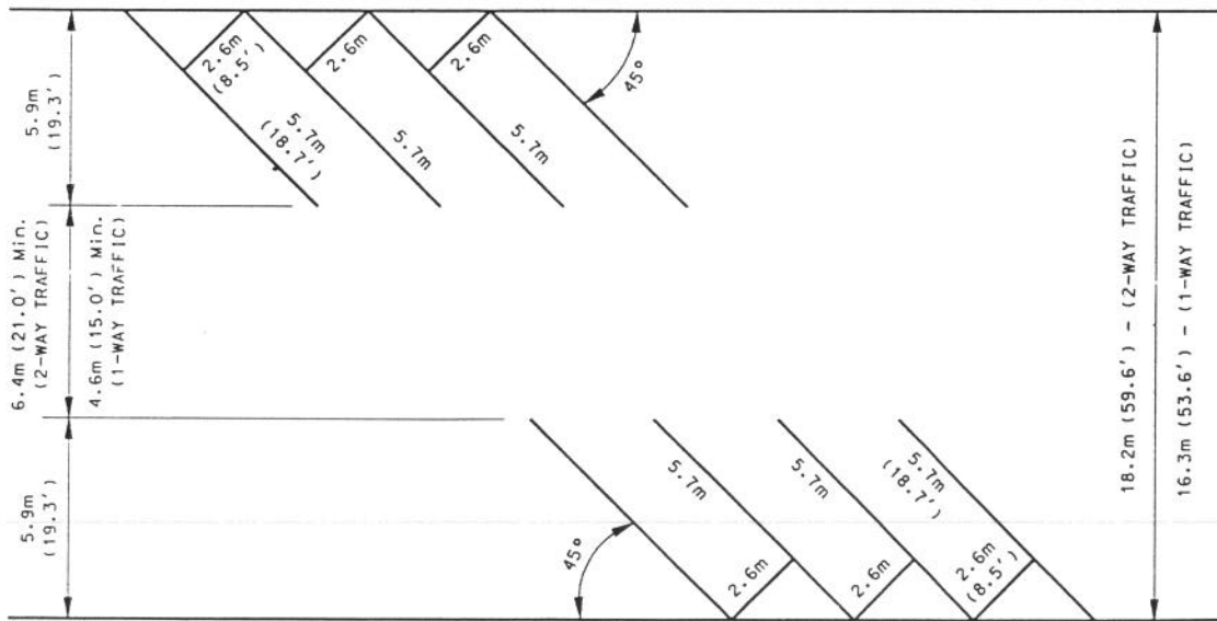
D) 45° ANGLE PARKING
