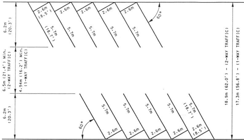
C) 60° ANGLE PARKING
